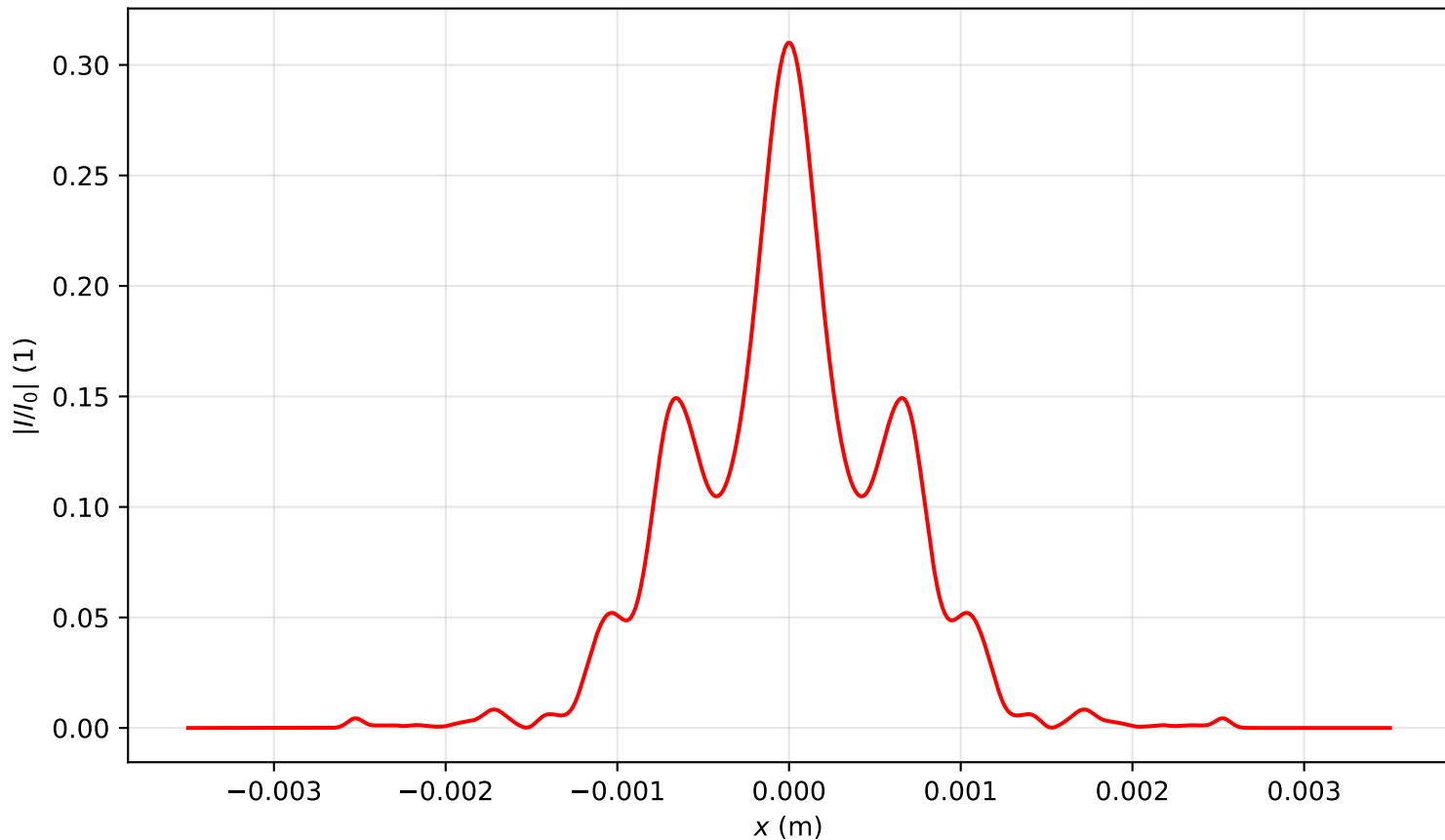
Intensity profile I(x, y = 0, z = 1.911)/I_0 , P_{in}=6.5P_{cr} , artificial time
